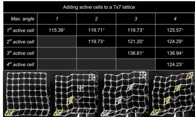
Figure 13: The max. achievable angle of our active cells increases when using multiple to drive the 7 \times 7 horizontal lattice. For example, the max. angle of the first active cell increases from 115.39^\circ with only one active cell to 125.57^\circ with four active cells. This indicates that the increasing resistance of larger lattices can be overcome by adding more active cells.
