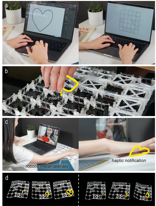
Figure 20: (a) A user designs a heart path for their haptic notification, and receives cell configuration from our software. (b) They insert cells as shown in the software. (c) When video-chatting with a friend, Robotic Metamaterials integrated into their desk renders a heart shape on their palm. (d) The same Robotic Metamaterials configuration is able to draw other symbols, such as a water drop.
