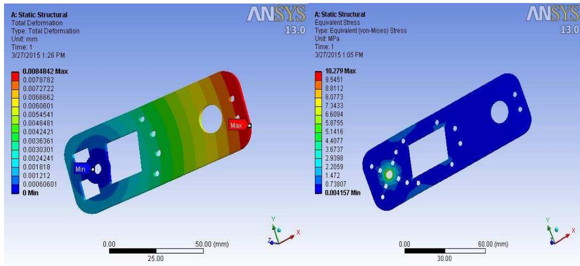
Figure 15: Total Deformation of Elbow
